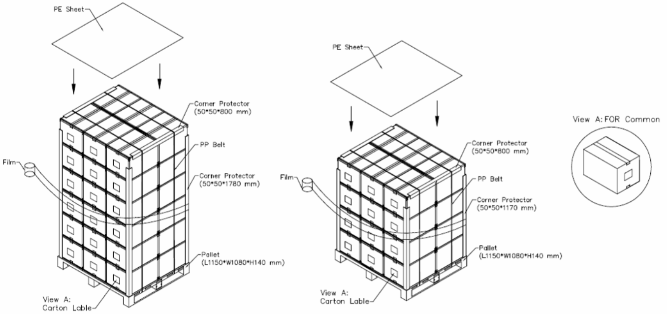
Figure. 7-3 Packing method
