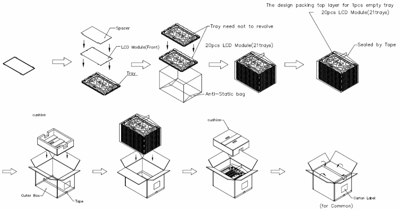
Figure. 7-2 Packing method
