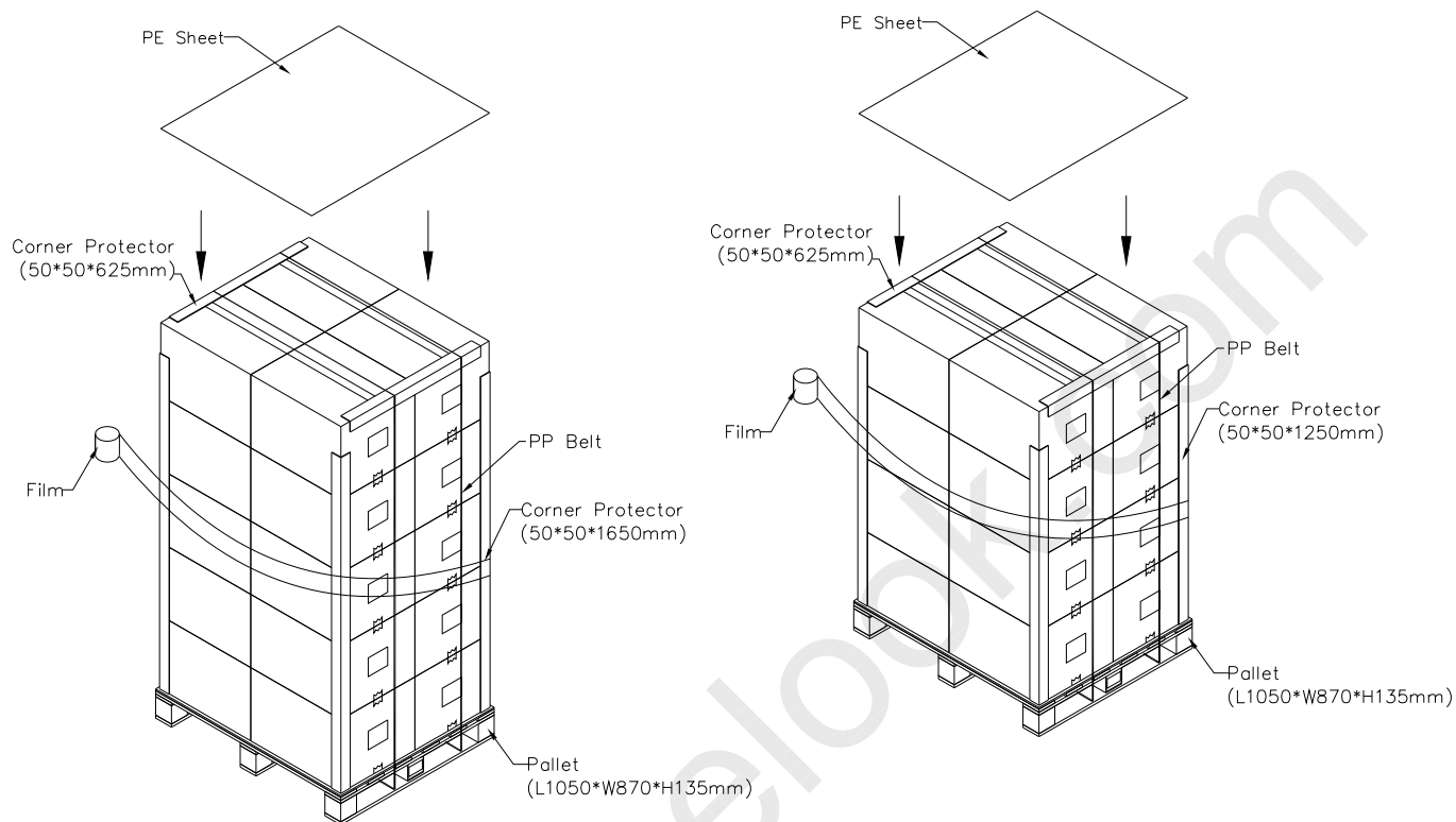
Figure. 7-3 Packing
