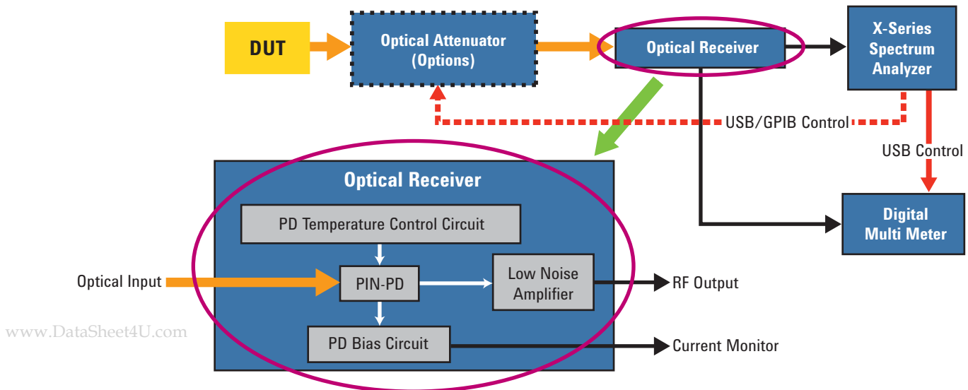
Figure 3. RIN Measurement System Block Diagram
