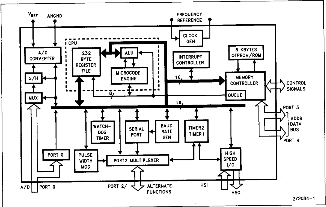
Figure 1. 87C198 Block Diagram
