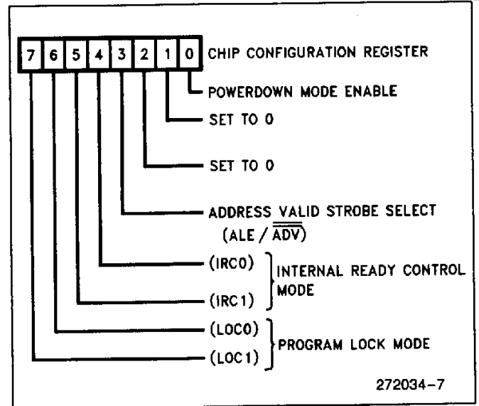
Figure 3. Chip Configuration (2018H)
