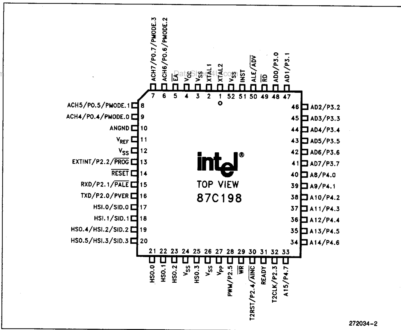
Figure 4. 52-Pin PLCC Package
