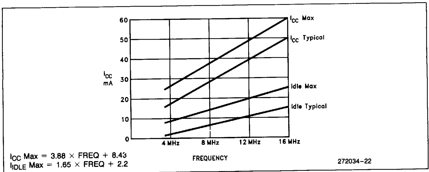
Figure 8. I_{CC} and I_{IDLE} vs Frequency
