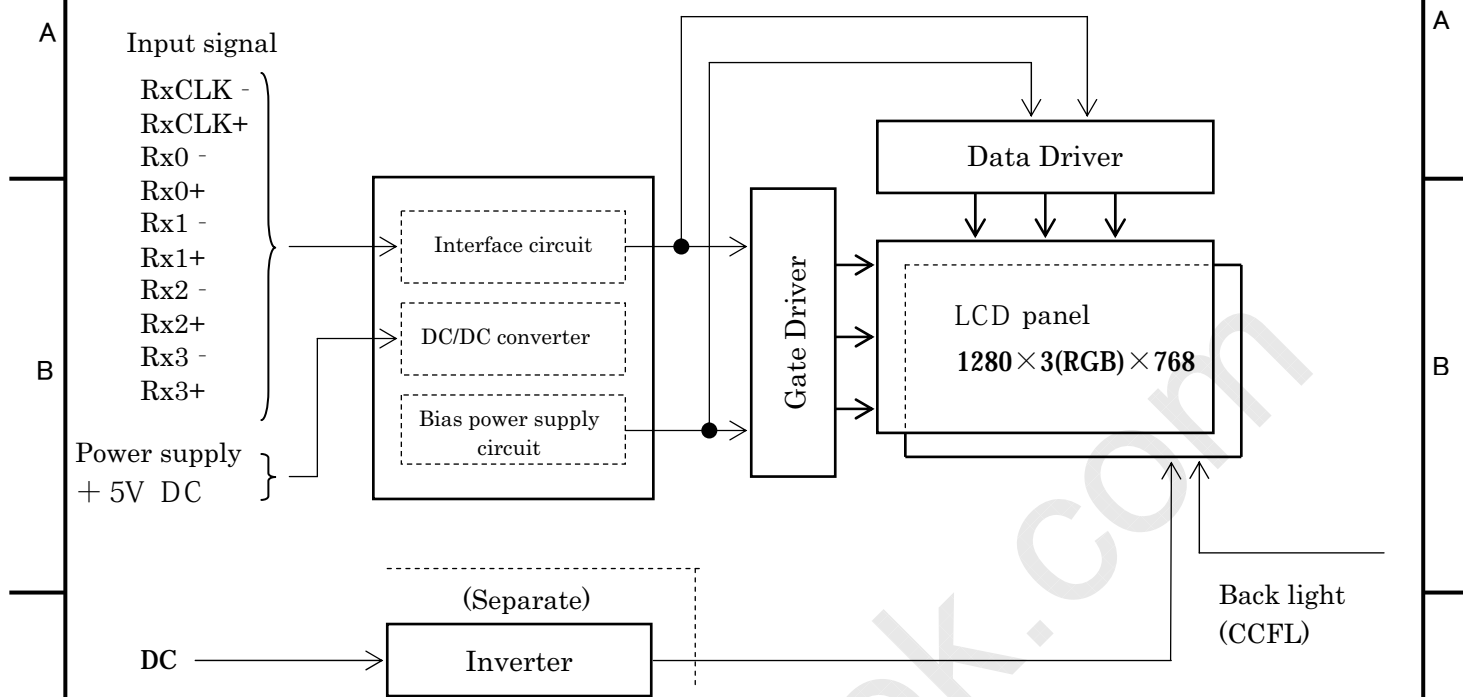
Figure 4-1. Block Diagram
