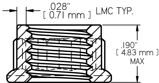
SECTION A-A 6X SCALE
