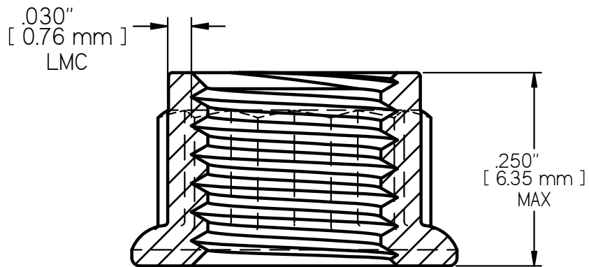
SECTION A-A 6X SCALE
