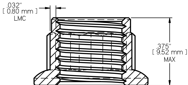
SECTION A-A 4X SCALE
