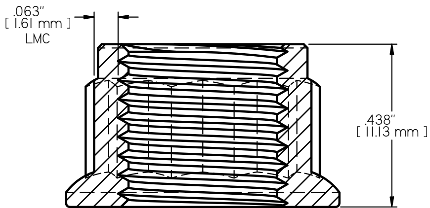
SECTION A-A 4X SCALE
