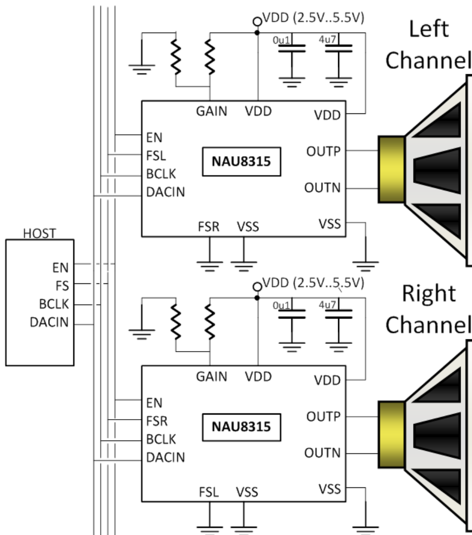
Figure 17 NAU8315/NAU83U15 Simplified System Diagram
