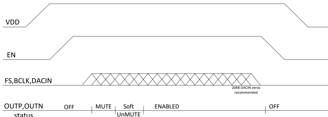
Figure 5 NAU8315/NAU83U15 Power Up & Down Sequence
