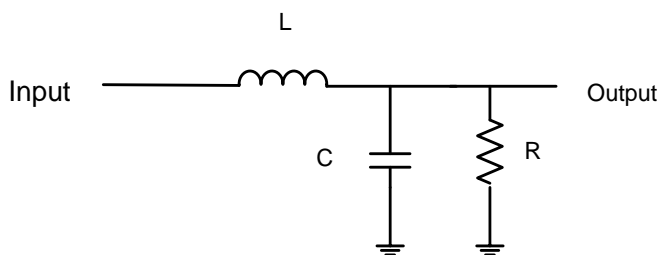
Figure 12 NAU8315/NAU83U15 Speaker Connections with Low-Pass Filters
