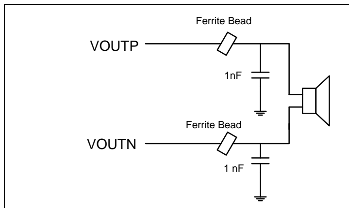
Figure 10 NAU8315/NAU83U15 Speaker Connections with Ferrite Bead Filters
