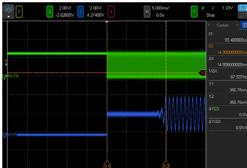
Figure 7 PWRUPEN startup sequence.
