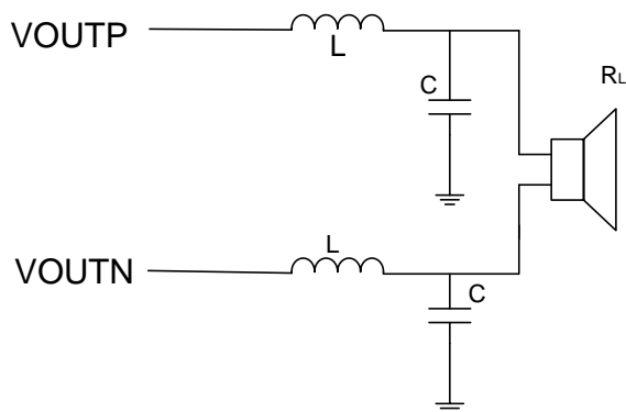
Figure 11 NAU8315/NAU83U15 Speaker Connections with LC Filters
