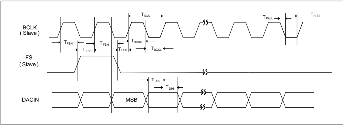
Figure 15 I2S Audio Interface
