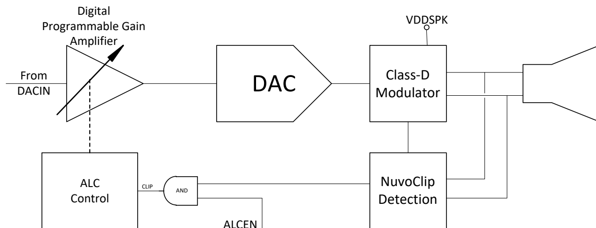
Figure 8 ALC Control Loop Block Diagram
