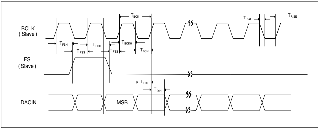
Figure 16 PCM Audio Interface
