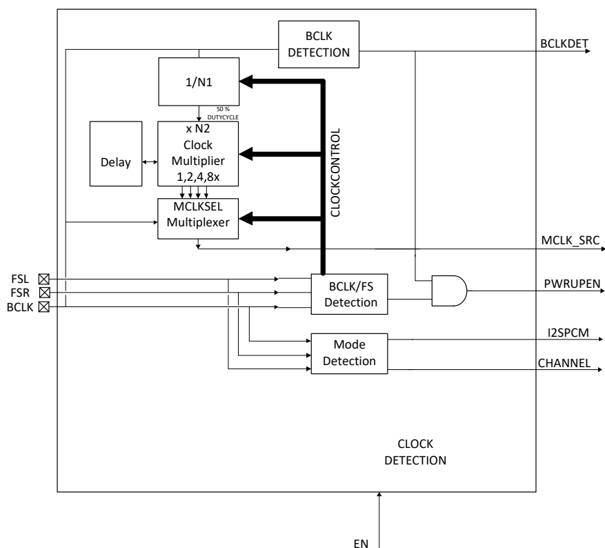
Figure 6 NAU8315/NAU83U15 Clock Detection Circuit
