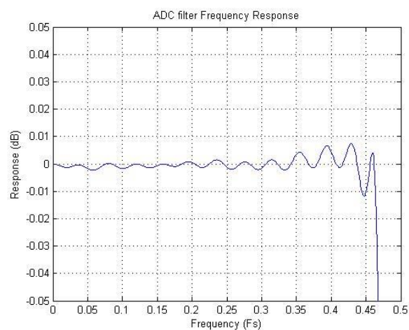
Figure 41: ADC Filter Ripple
