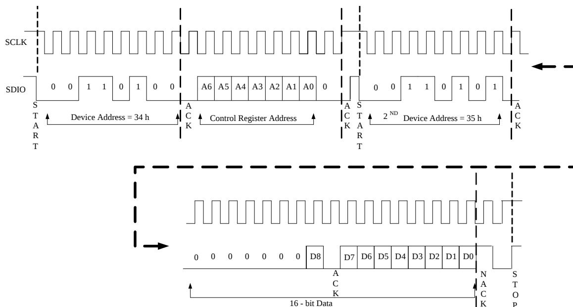
Figure 20: 2-Wire Read Sequence
