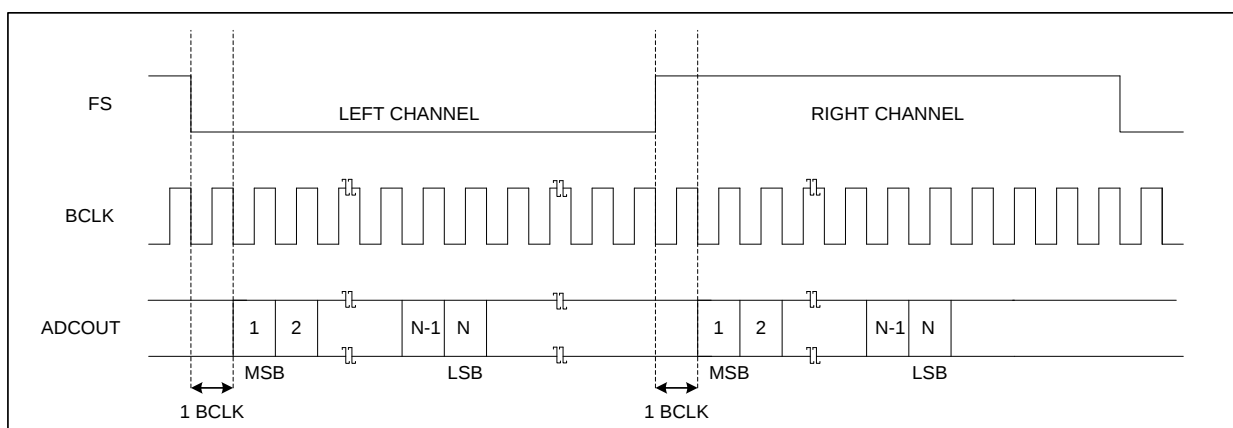
Figure 26: I2S Audio Interface (Special mode)
