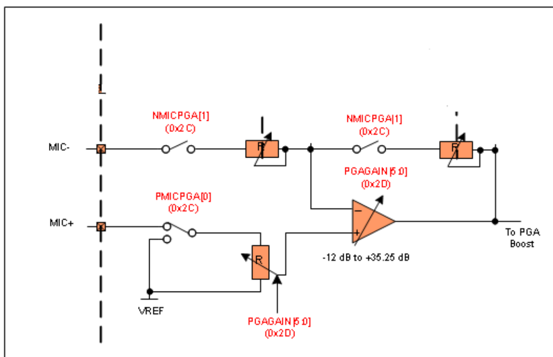
Figure 3: Input PGA Circuit Block Diagram
