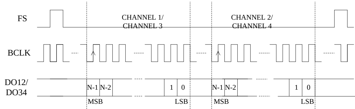
Figure 24: PCM Time Slot Audio Format
