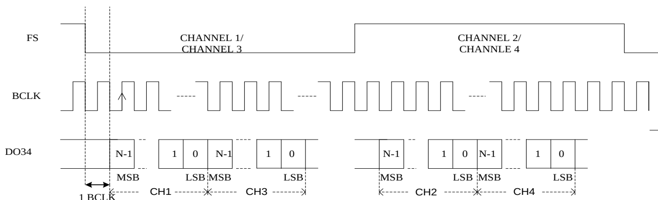
Figure 33: TDM I2S Audio Format
