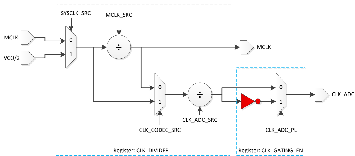
Figure 9: Clock Generation
