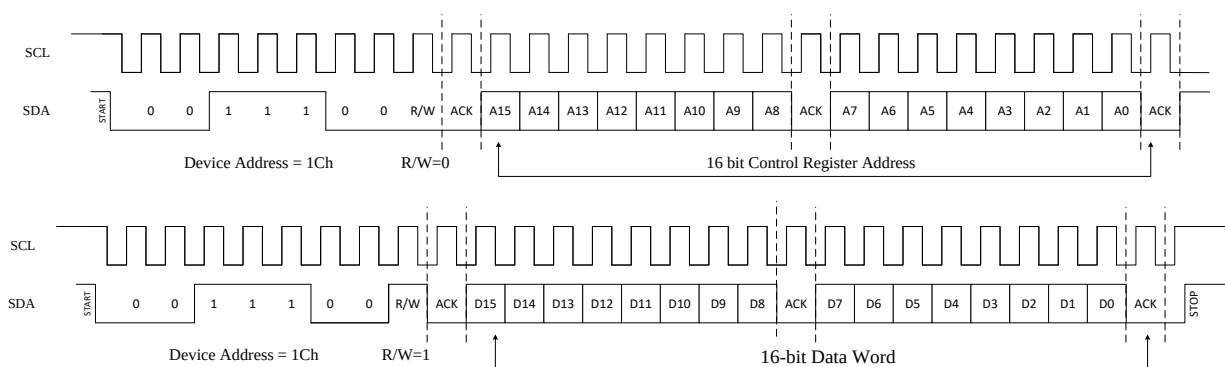
Figure 17: Read Sequence
