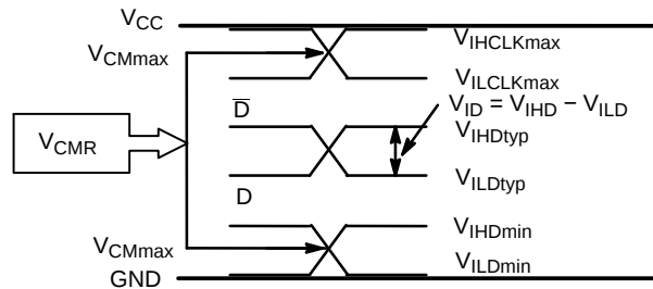
Figure 17. V_{CM} Diagram
