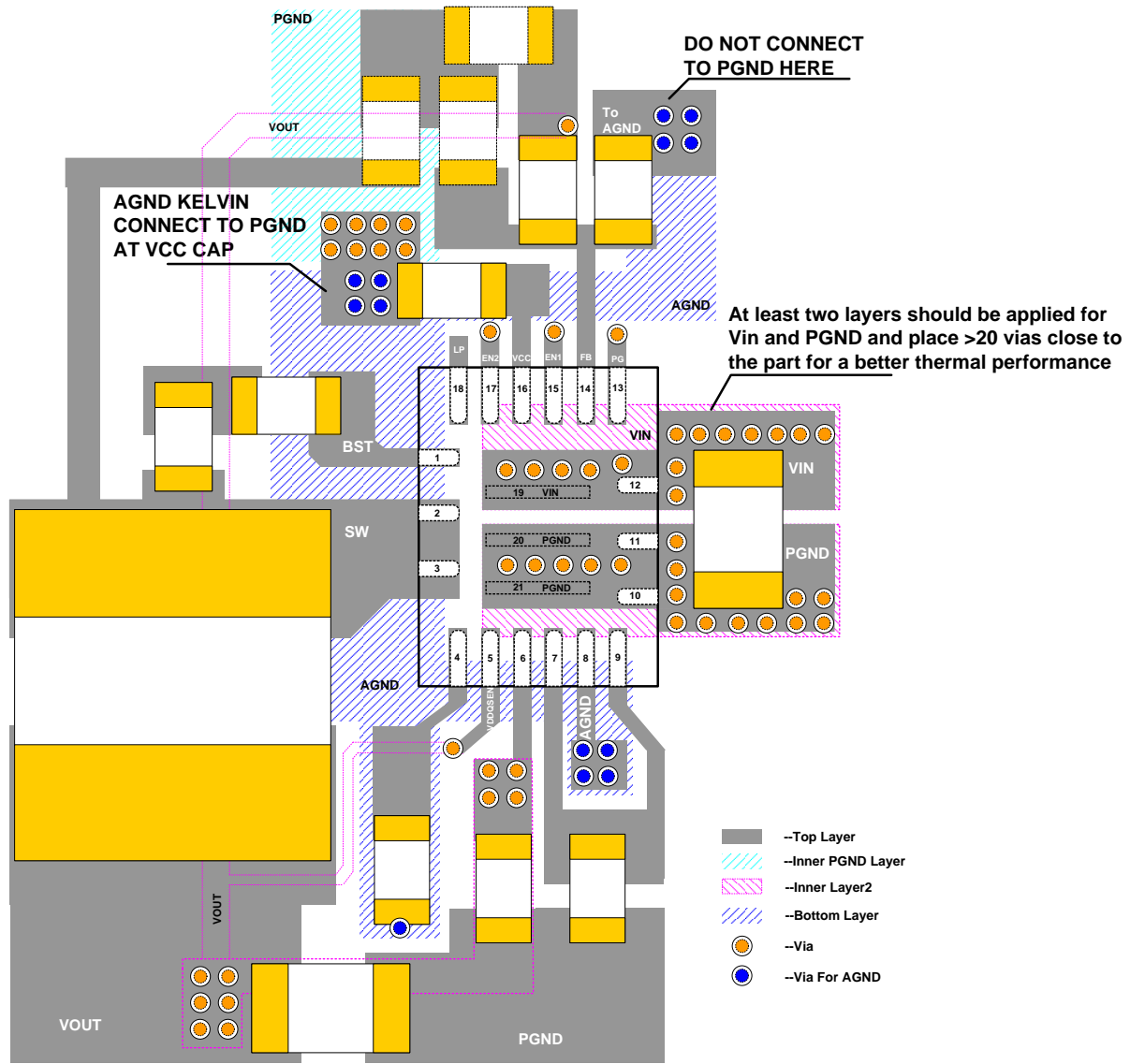
Figure 13—Recommend Layout
