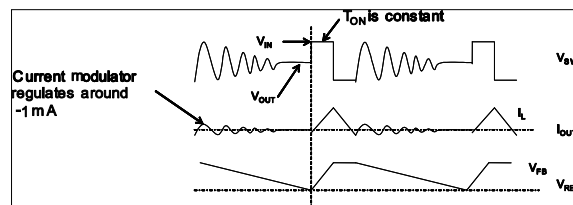
Figure 3—DCM Operation
