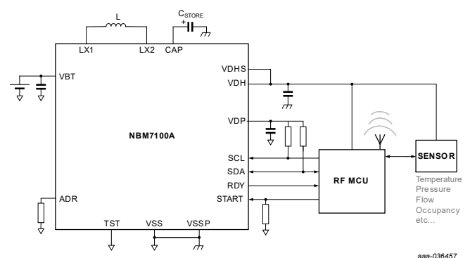
Fig. 2. Simplified Application
