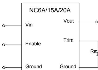
Figure 27: Trimming Output Voltage DS_NC12S06A_02072007
