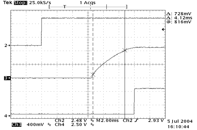
Figure 14: Turn on delay Remote On/Off, 0.9V/6A out Ch2: ENABLE Ch3: Vout Ch4: PWRGD
