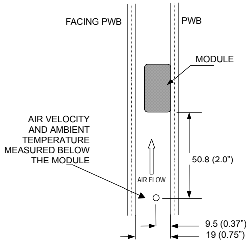
Note: Wind Tunnel Test Setup Figure Dimensions are in millimeters and (Inches) Figure 38: Wind tunnel test setup
