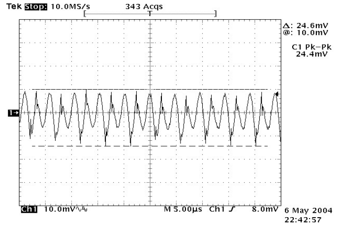
Figure 10: Output ripple & noise at 12Vin, 2.5V/20A out
