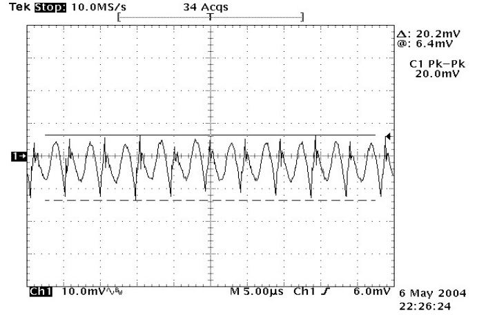
Figure 8: Output ripple & noise at 12Vin, 1.2V/20A out
