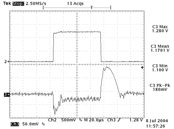
Figure 20: Typical transient response to step load change at 10A/µs from 50% to 75% and 75% to 50% of I_{o\_max} at 12Vin, 1.2V out
