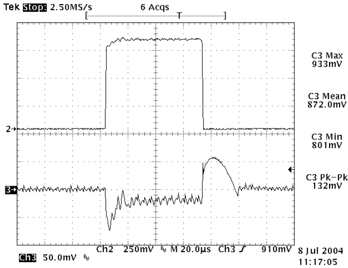
Figure 19: Typical transient response to step load change at 10A/µs from 50% to 75% and 75% to 50% of I_{o\_max} at 12Vin, 0.9V out
