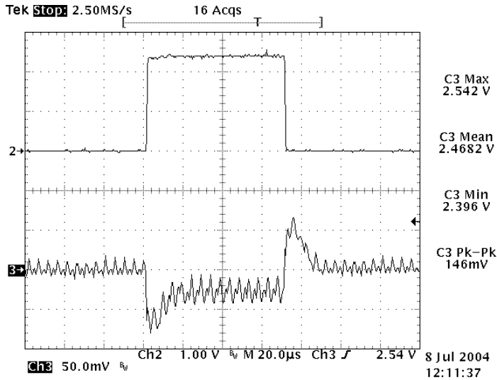
Figure 21: Typical transient response to step load change at 10A/µs from 50% to 75% and 75% to 50% of I_{o\_max} at 12Vin, 2.5V out
