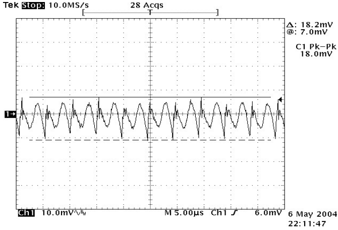
Figure 7: Output ripple & noise at 12Vin, 0.9V/20A out
