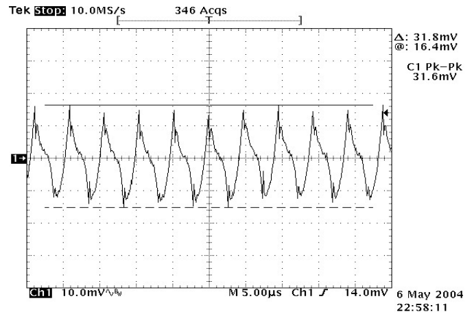
Figure 12: Output ripple & noise at 12Vin, 5.0V/20A out
