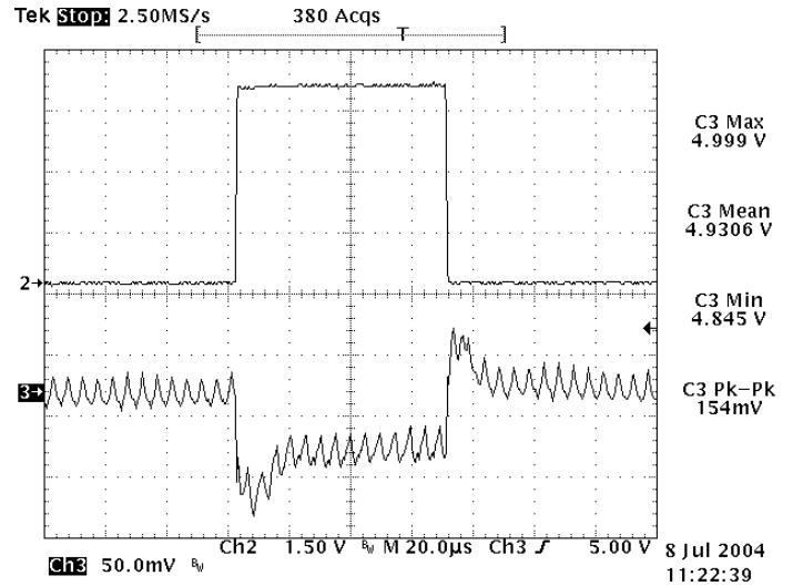
Figure 22: Typical transient response to step load change at 10A/µs from 50% to 75% and 75% to 50% of I_{o\_max} at 12Vin, 5.0V out
