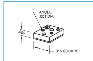
CH3 Chip (inches)
