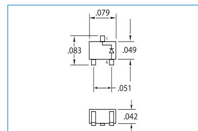
SOT323 Package (inches)
