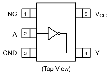
Figure 2. Connection Diagram
