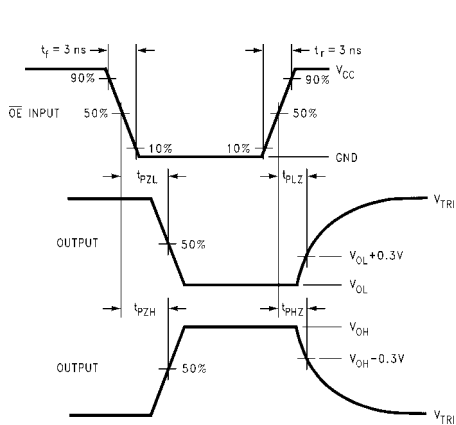
FIGURE 4. AC Waveforms
