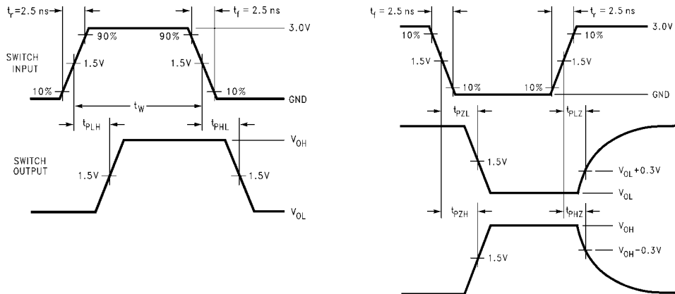
FIGURE 2. AC Waveforms
