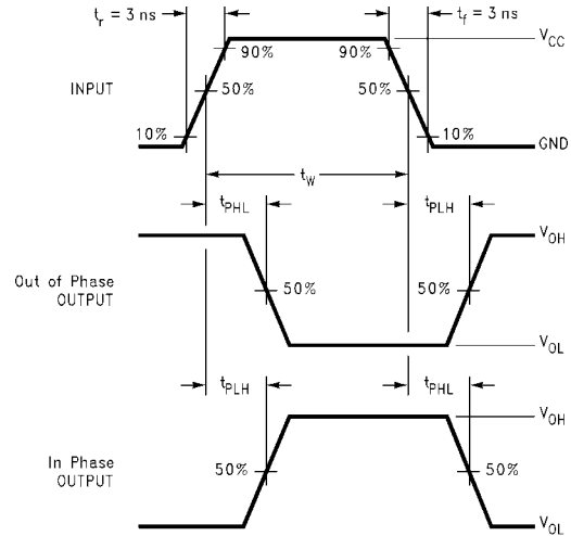
FIGURE 3. AC Waveforms
