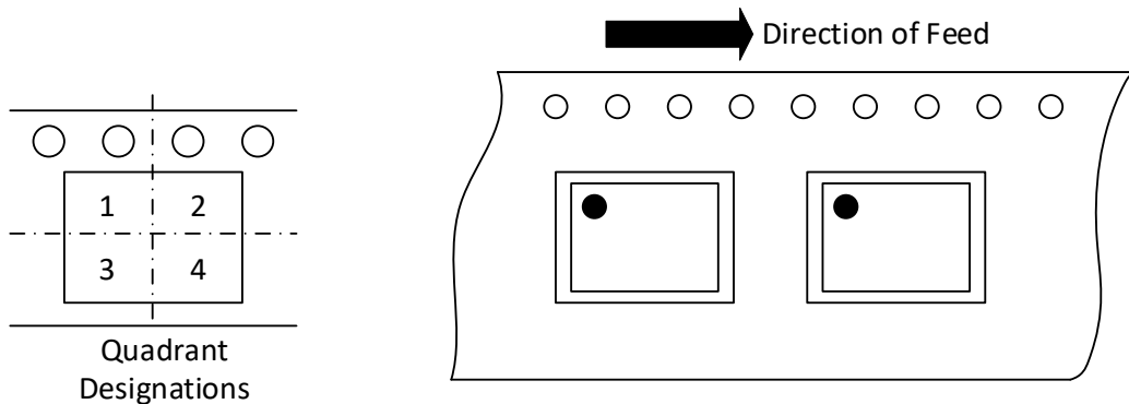
Figure 12-1. Tape and reel information for TSSOP24
