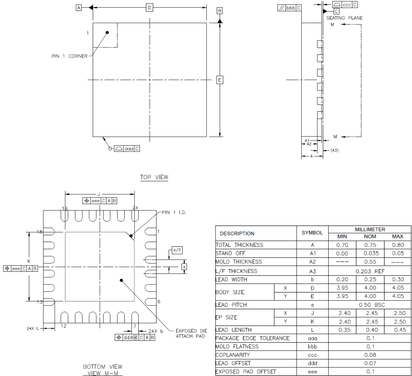
Figure 11-4. QFN24 Package Shape and Dimension in millimeters
