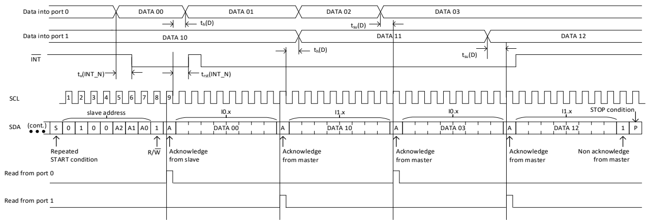
Figure 7-12. Read input port registers, scenario 1
