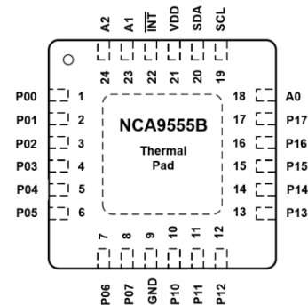
Figure 2. NCA9555B-DQNXR Pinout
