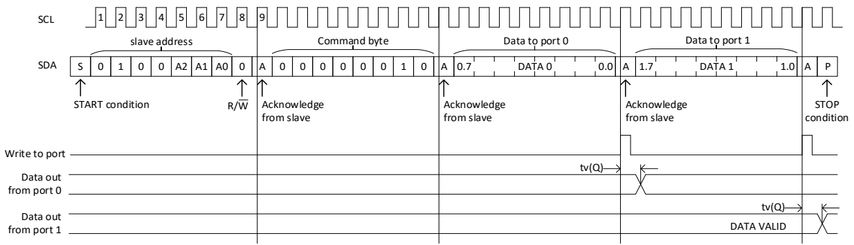
Figure 7-9. Write to output port registers
