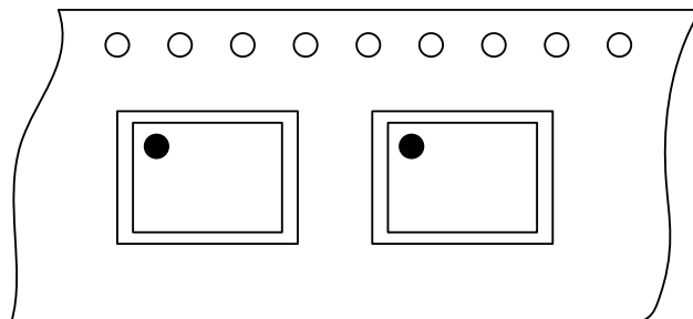
Figure 12-2. Tape and reel information for QFN24
