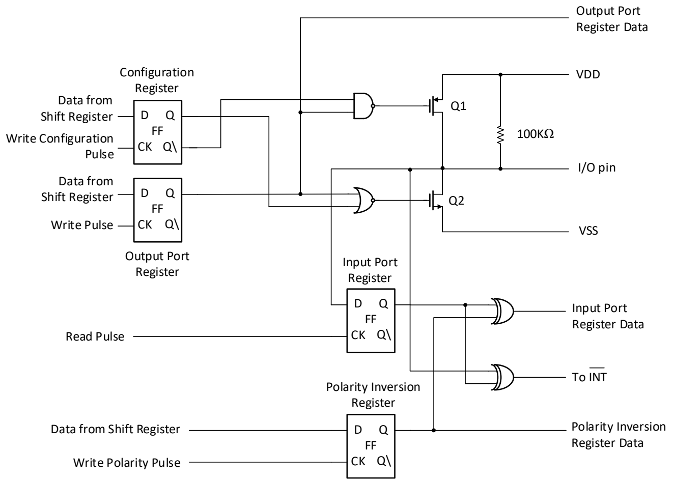
Figure 7-2. Simplified schematic of I/Os
