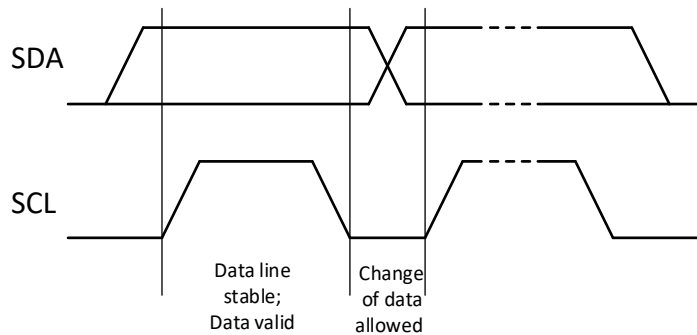
Figure 7-4. Bit transfer
