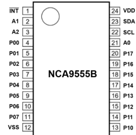
Figure 1. NCA9555B-DTSXR Pinout
