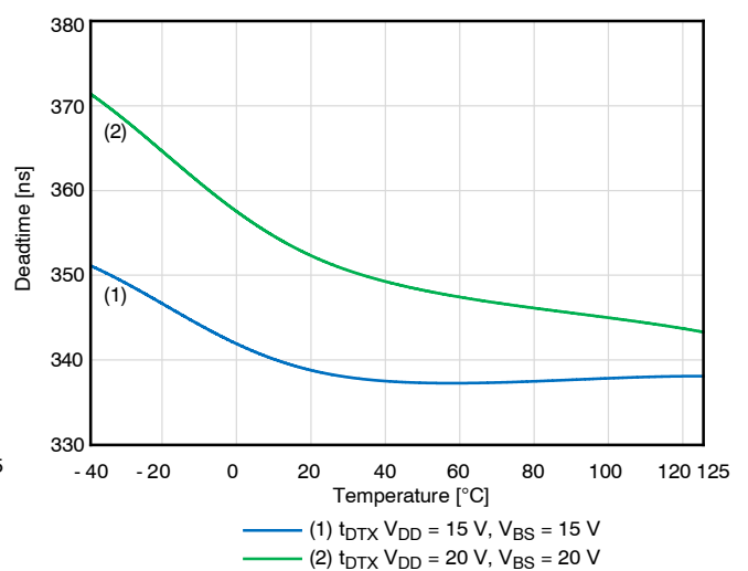
Figure 25. Deadtime
