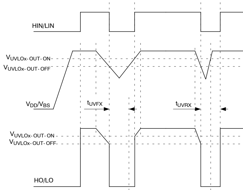
Figure 5. UVLO
