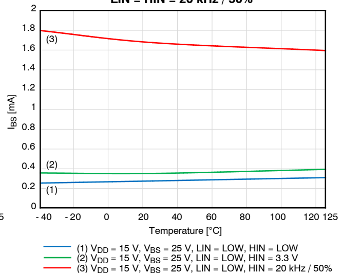
Figure 13. I_{BS} Supply Current V_{BS} = 25\text{ V}
