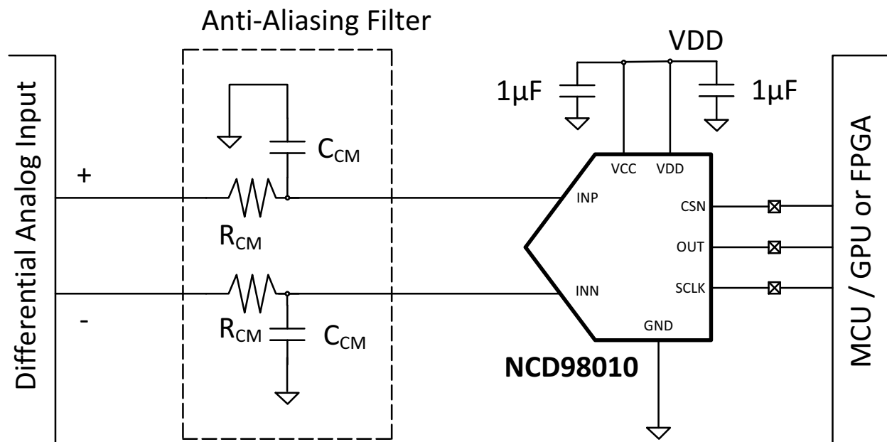
Figure 21. Reduced Component Connection Diagram
