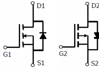
N-channel P-channel
