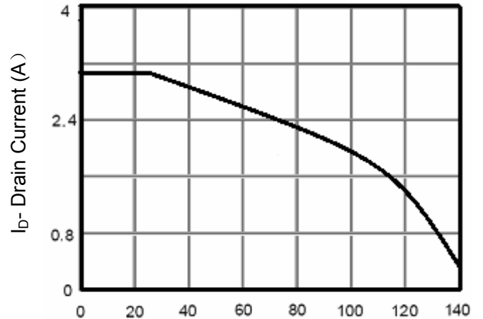
Figure 4 Drain Current
