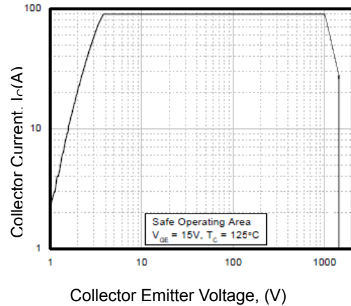
Figure 16. Turn-Off SOA
