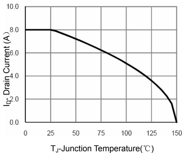
Figure 4 Drain Current
