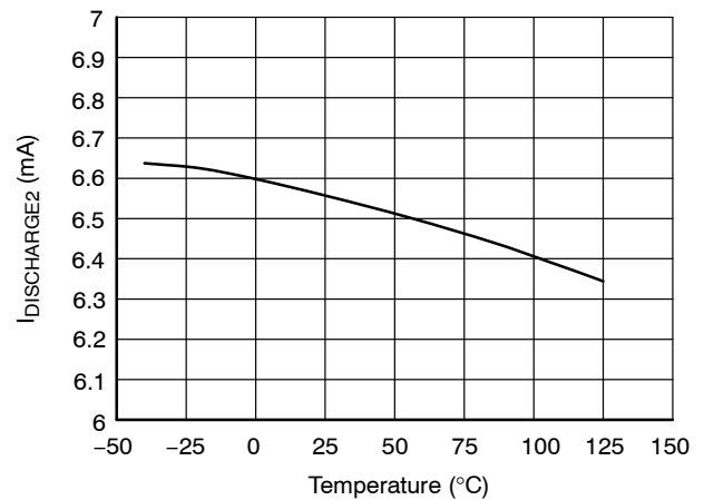
Figure 14. HB Sink Current Capability @ V_{HB} = V_{HB\_MIN}
