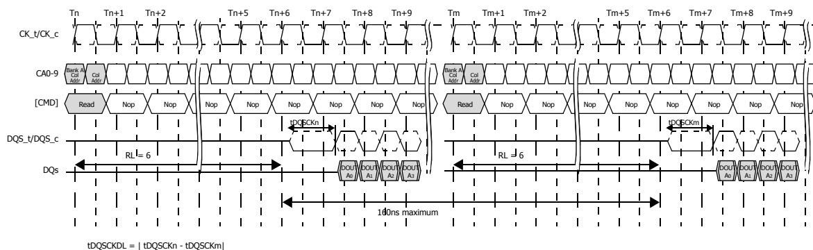
Figure. LPDDR3 : tDQSKDS timing
