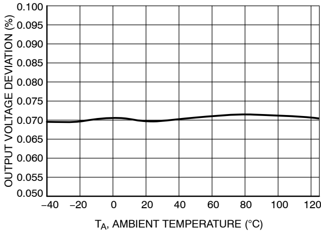
Figure 6. Line Regulation vs. Temperature I load = 10 mA
