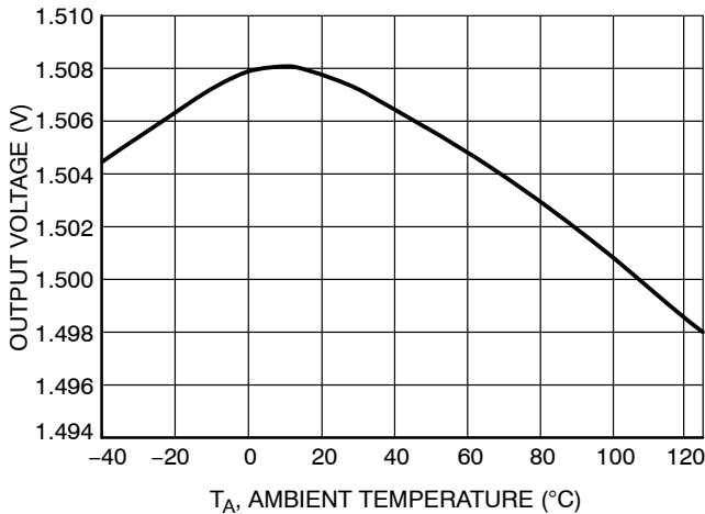
Figure 8. Output Voltage vs. Temperature I load = 10 mA
