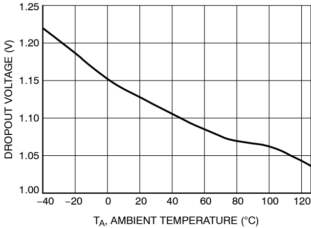
Figure 4. Dropout Voltage vs. Temperature I load = 10 mA
