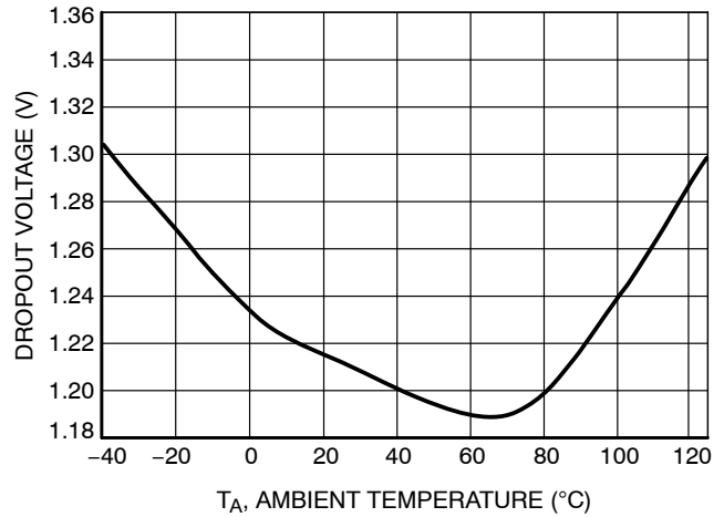
Figure 5. Dropout Voltage vs. Temperature I load = 1 A
