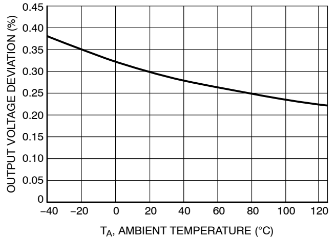
Figure 7. Load Regulation vs. Temperature I load = 1 A
