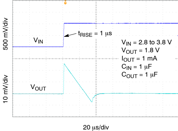
Figure 14. Line Transient Response – Rising Edge
