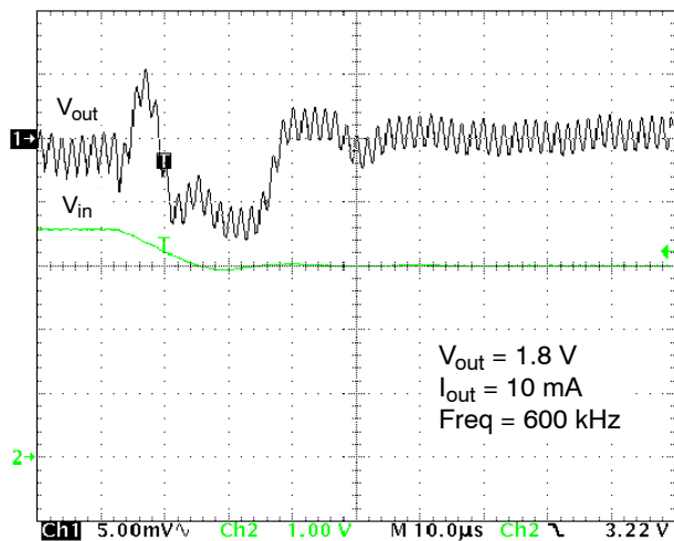
Figure 27. Line Transient from 3.6 to 3.0 V
