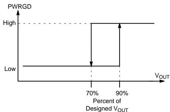
Figure 23. PWRGD Assertion
