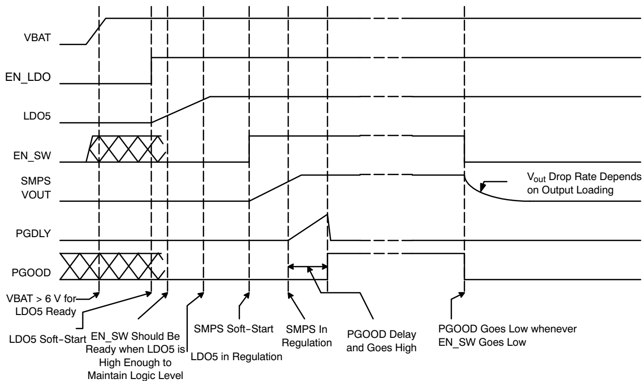
Figure 33. Single V BAT Configuration (SMPS Disabled by EN_SW)
