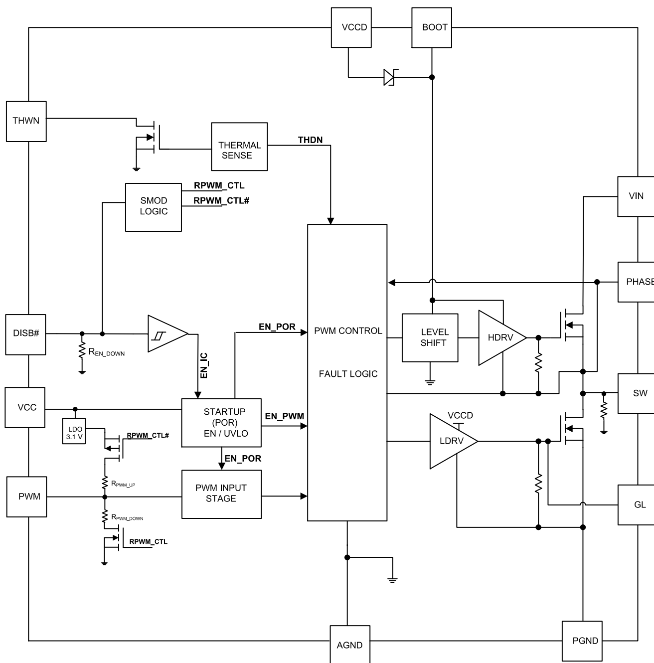
Figure 2. Block Diagram
