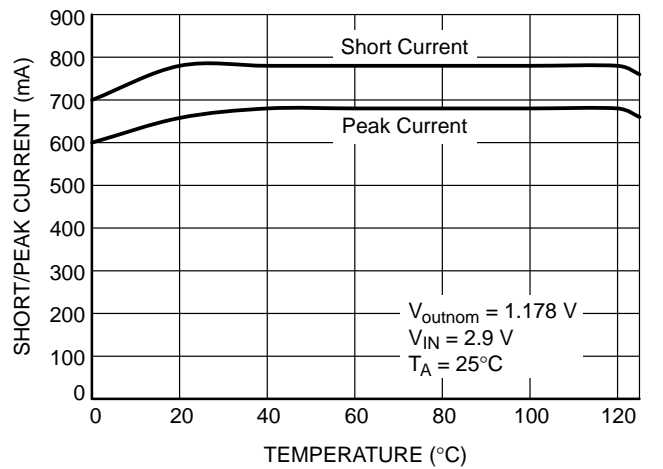
Figure 7. Peak and Short Current vs. Temperature
