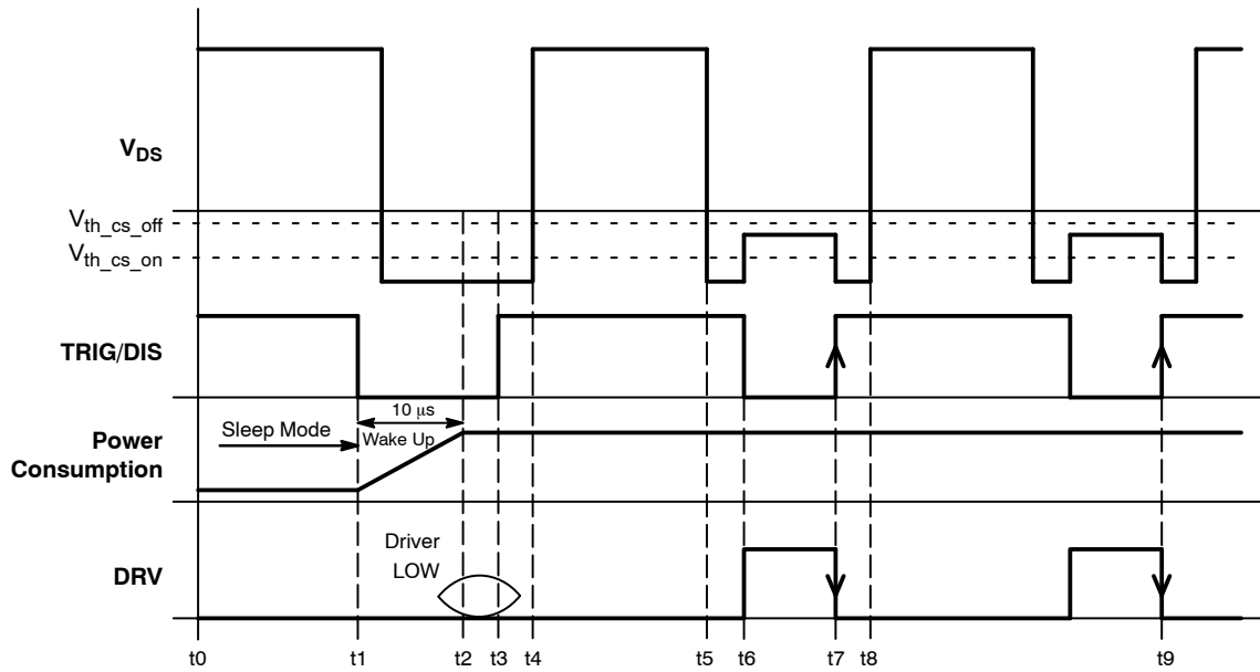
Figure 57. Waking-up Sequence
