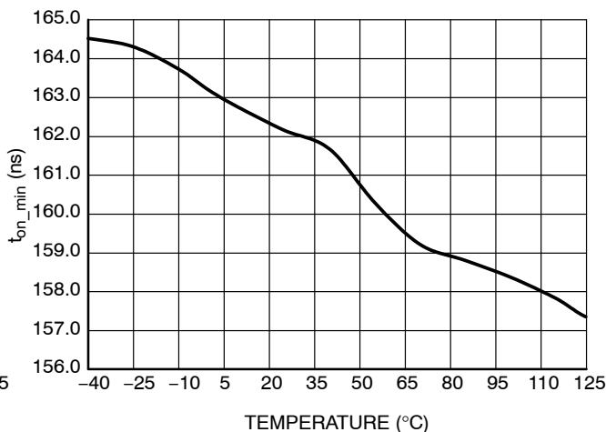
Figure 28. Minimum on Time @ R MIN_TON = 0 Ω
