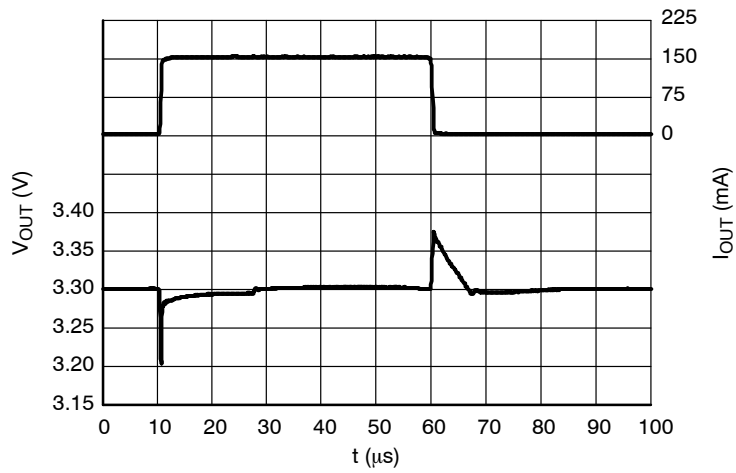
Figure 46. Load Transients, 3.3 V Version, I_{OUT} = 1 - 150 mA, t_R = t_F = 0.5 µs, V_{IN} = 4.3 V
