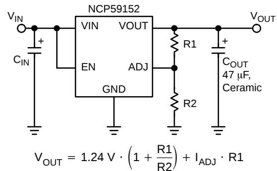
Figure 19. Adjustable Voltage Operation
