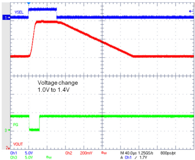
Figure 27. DVS Transition 1.0V – 1.39375 V
