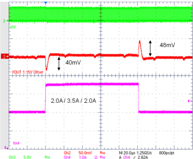
Figure 32. Transient Load 2.0 – 3.5 A Auto Mode
