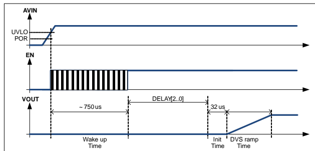
Figure 34. Initial Power Up Sequence
