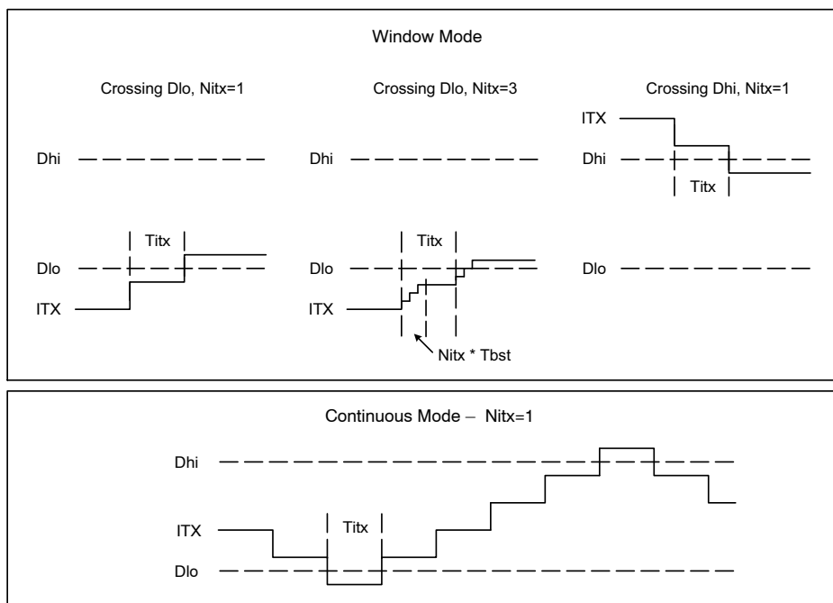
Figure 71. Discriminator Functionality
