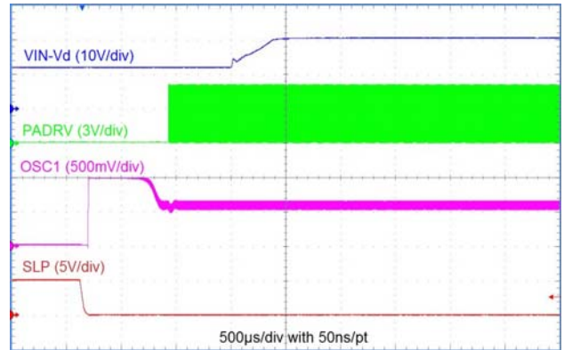
Figure 54. Oscillator, PA Boost and PA Driver Enabling Timing Out to Sleep Mode
