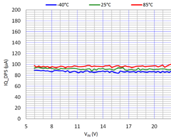
Figure 6. Deep Power Save Current vs. V_{IN} (V)
