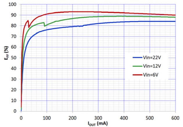
Figure 13. Buck Converter Efficiency
