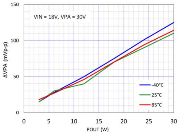
Figure 30. Boost Converter Output Voltage Ripple vs. P_{OUT}
