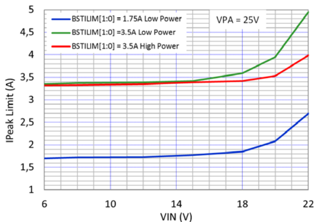
Figure 25. Boost Converter I_{peak} Limit vs. V_{IN} (V)
