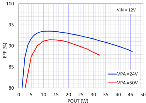
Figure 23. Boost Converter Efficiency vs. P_{OUT}
