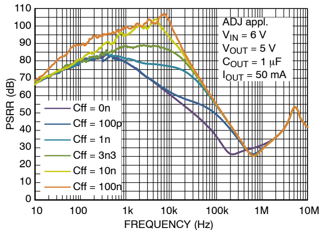
Figure 28. PSRR vs. C_{FF}
