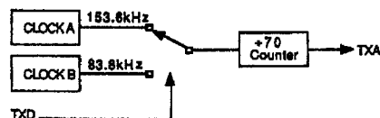
Modulator Block Diagram
