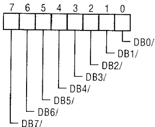
Input Data Register (3886H)
