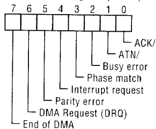
Interrupt Status Register (3885H)
