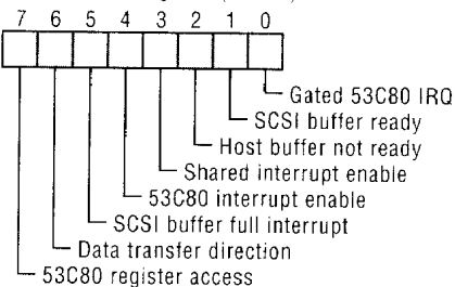
Control Status Register (3980H)
