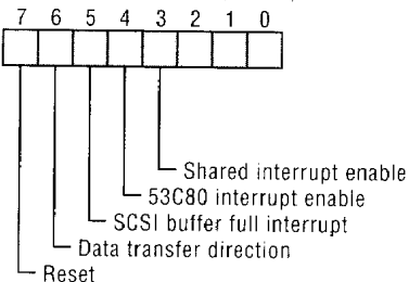
Control Status Register (3980H)
