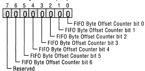
DFIFO Register R/W (20h)
