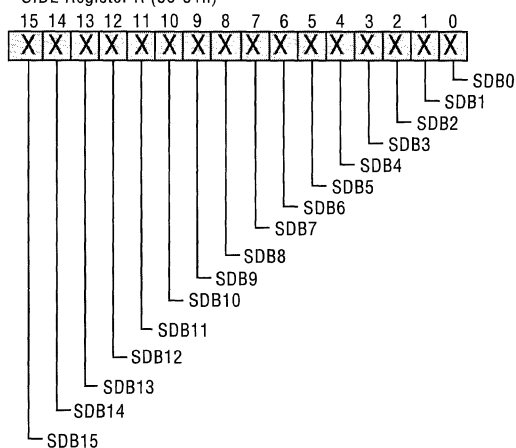
SIDL Register R (50-51h)
