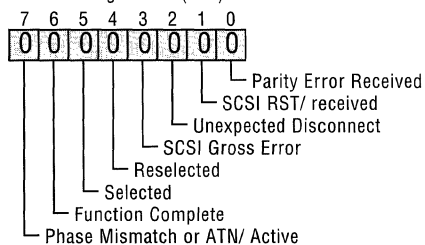
SIST0 Register R (42h)
