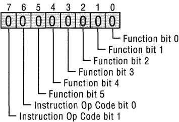
DCMD Register R/W (27h)
