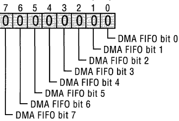
CTEST6 Register R/W (23h)
