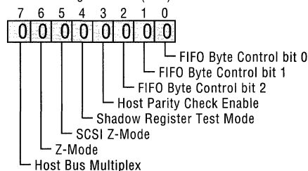
CTEST4 Register R/W (21h)
