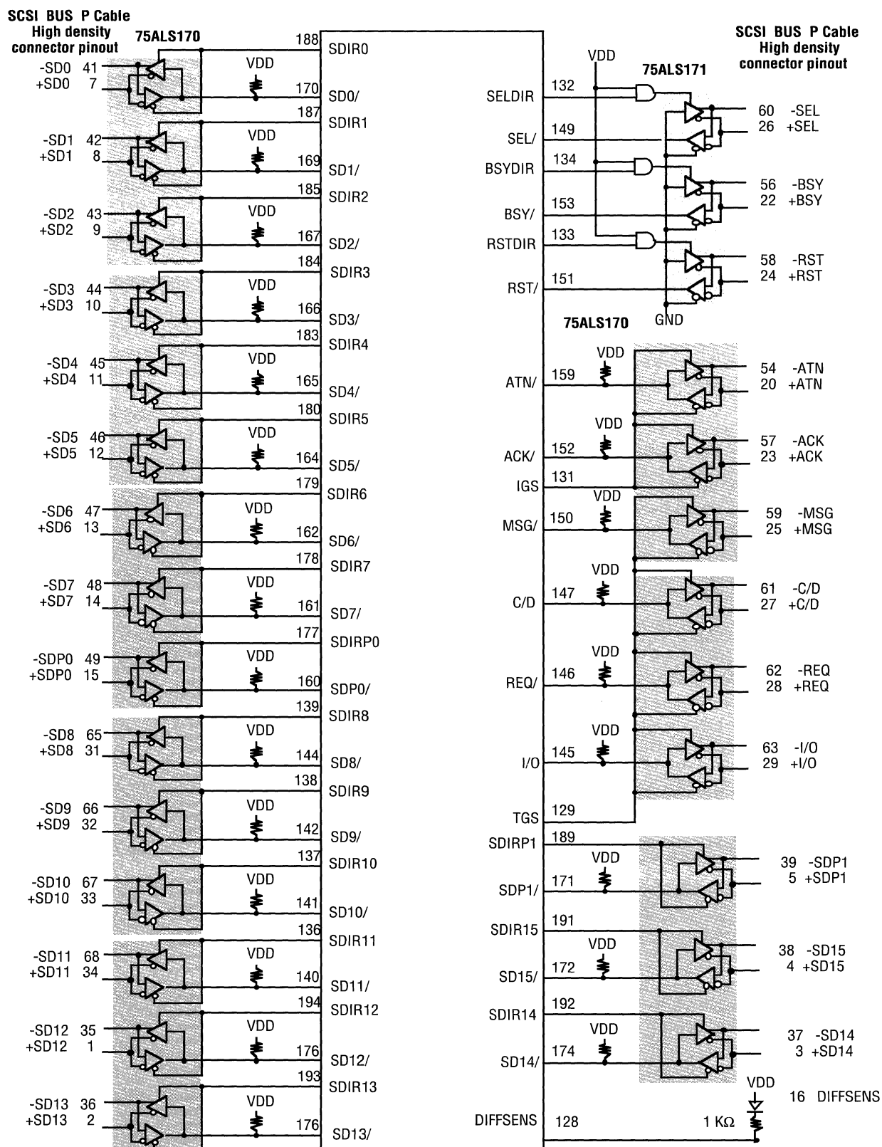
Figure 2-6. Differential Wiring Diagram
