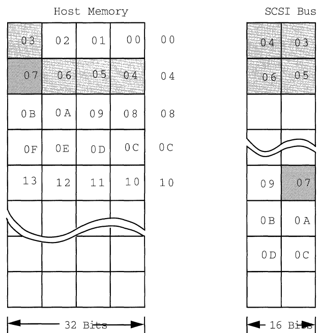
Figure 5-2. Block Move and Chained Block Move Instructions
