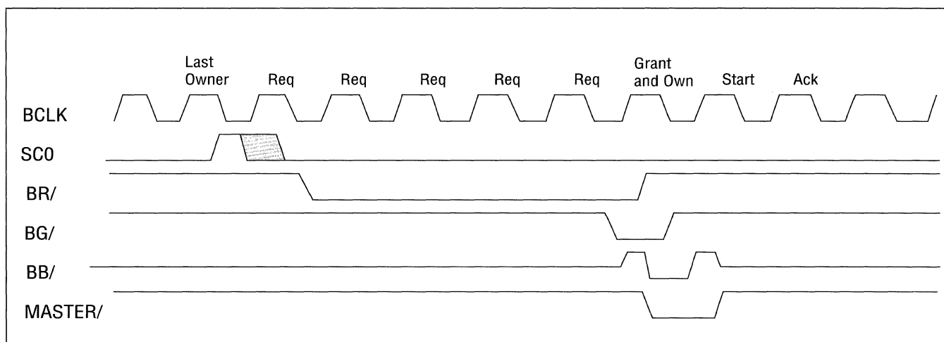
Figure 2. False Bus Request
