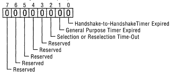
SIEN1 Register R/W (41h)
