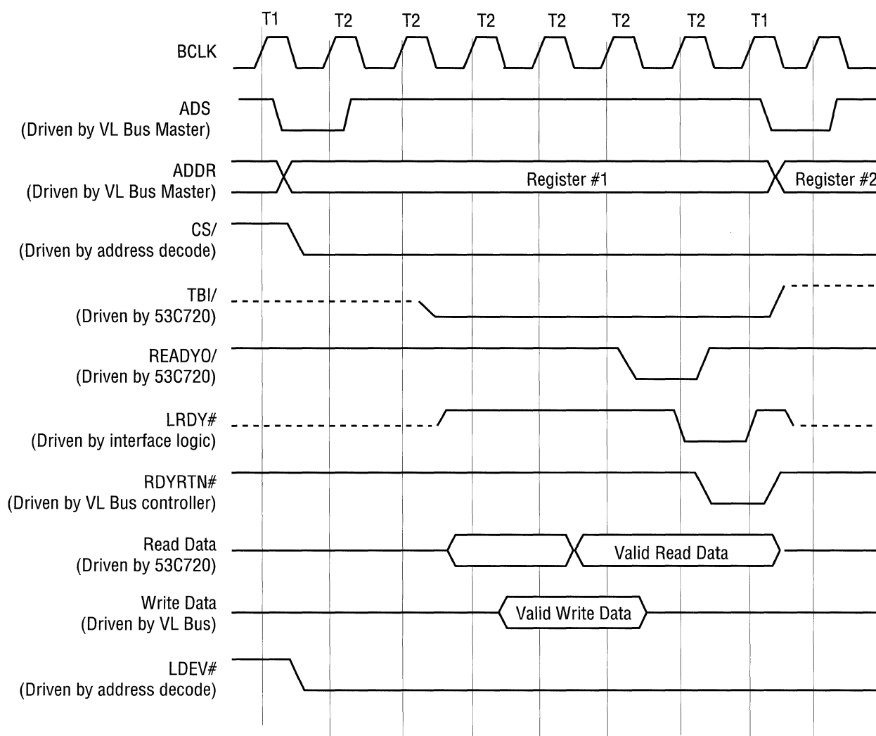
Figure 1. 53C720 and VL-Bus Slave Cycle
