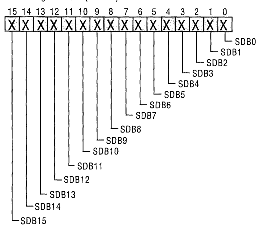
SODL Register R/W (54-55h)
