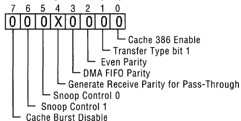
CTEST0 Register R/W (18h)
