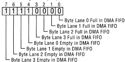
CTEST1 Register R (19h)
