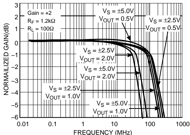
Figure 1. Frequency Response: Gain (dB) vs. Frequency A_V = +2.0
