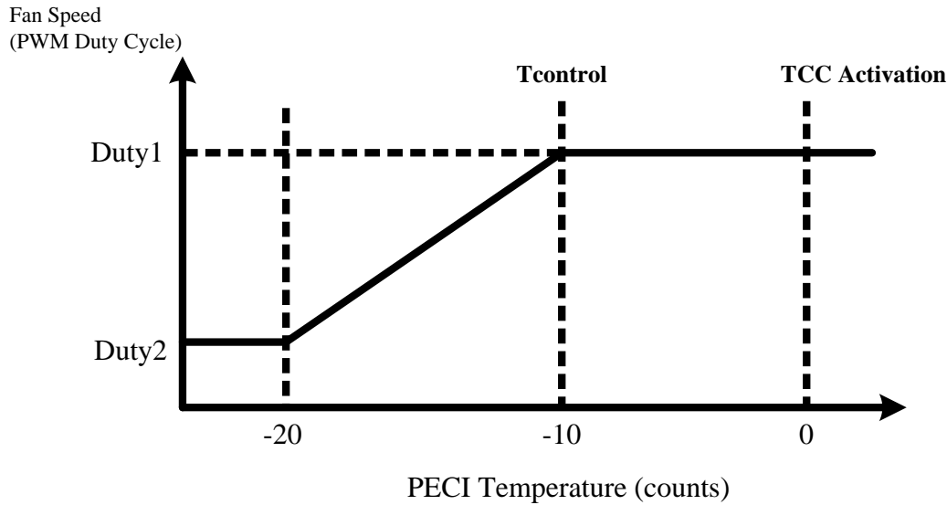
Figure 8-8 PECI Temperature
