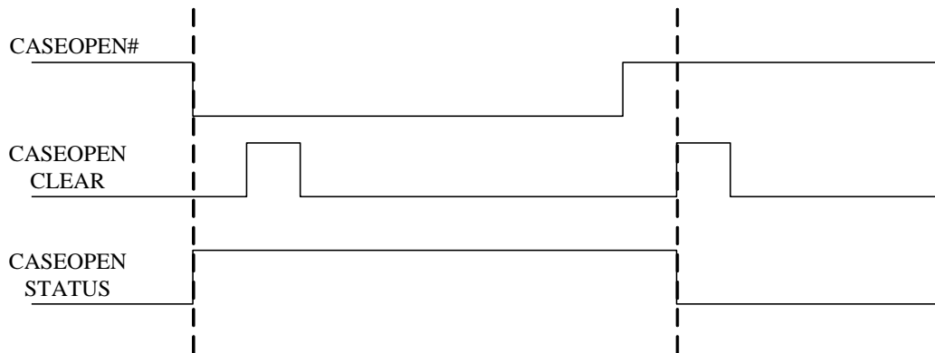
Figure 8-28 Caseopen Mechanism
